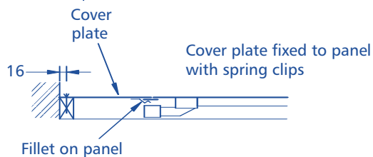
Cover Plate Detail
