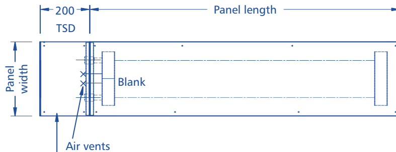
Plan
